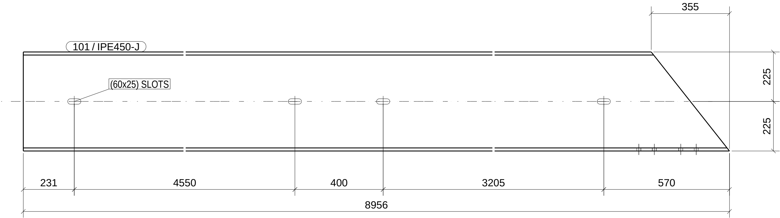
FRONT VIEW
