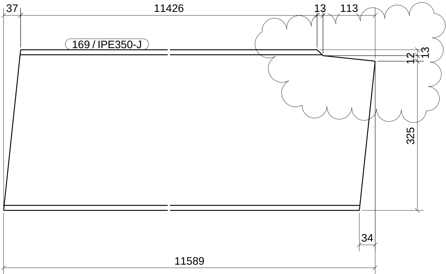
FRONT VIEW
