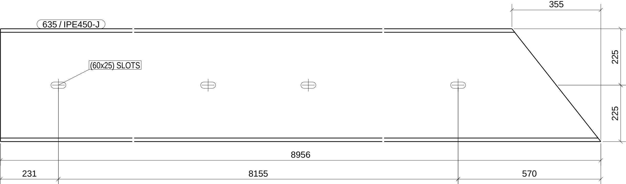
FRONT VIEW
